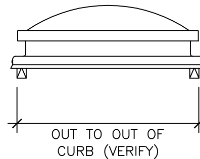
END ELEVATION NOT TO SCALE C —
