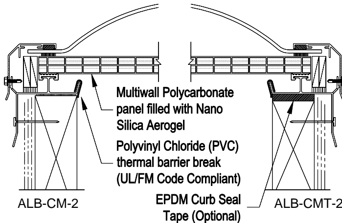
Acrylic Dome
