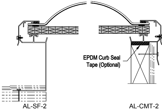
Polycarbonate Dome
