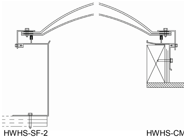
Polycarbonate Dome
