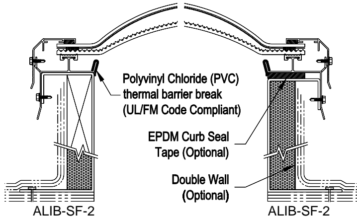
Acrylic Dome
