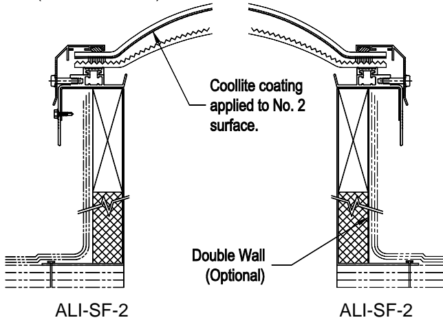
Acrylic/Polycarbonate Dome
