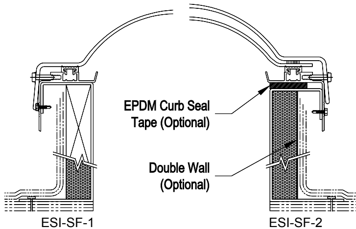
Fiberglass Dome
