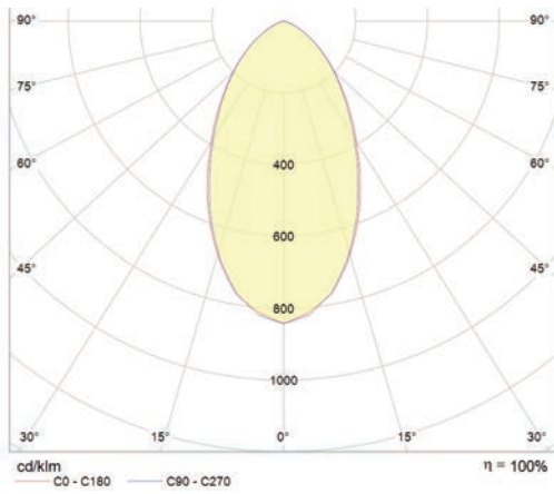
Wide 60°
