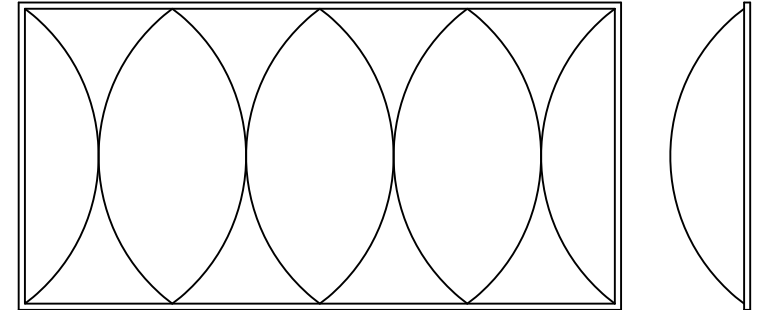
TRI-TUFF TRI-ARCH DOME DETAIL
