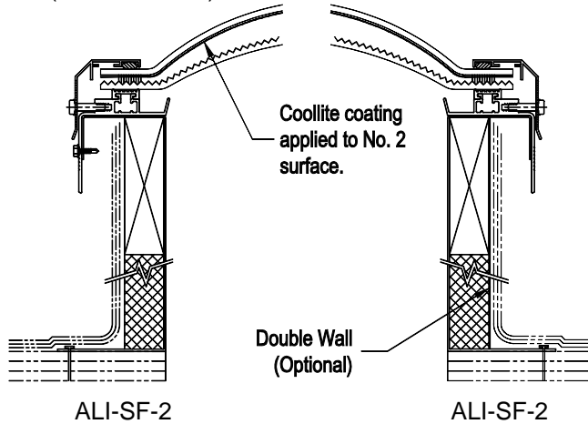
Acrylic/Polycarbonate Dome
