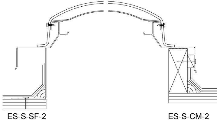
Fiberglass Dome
